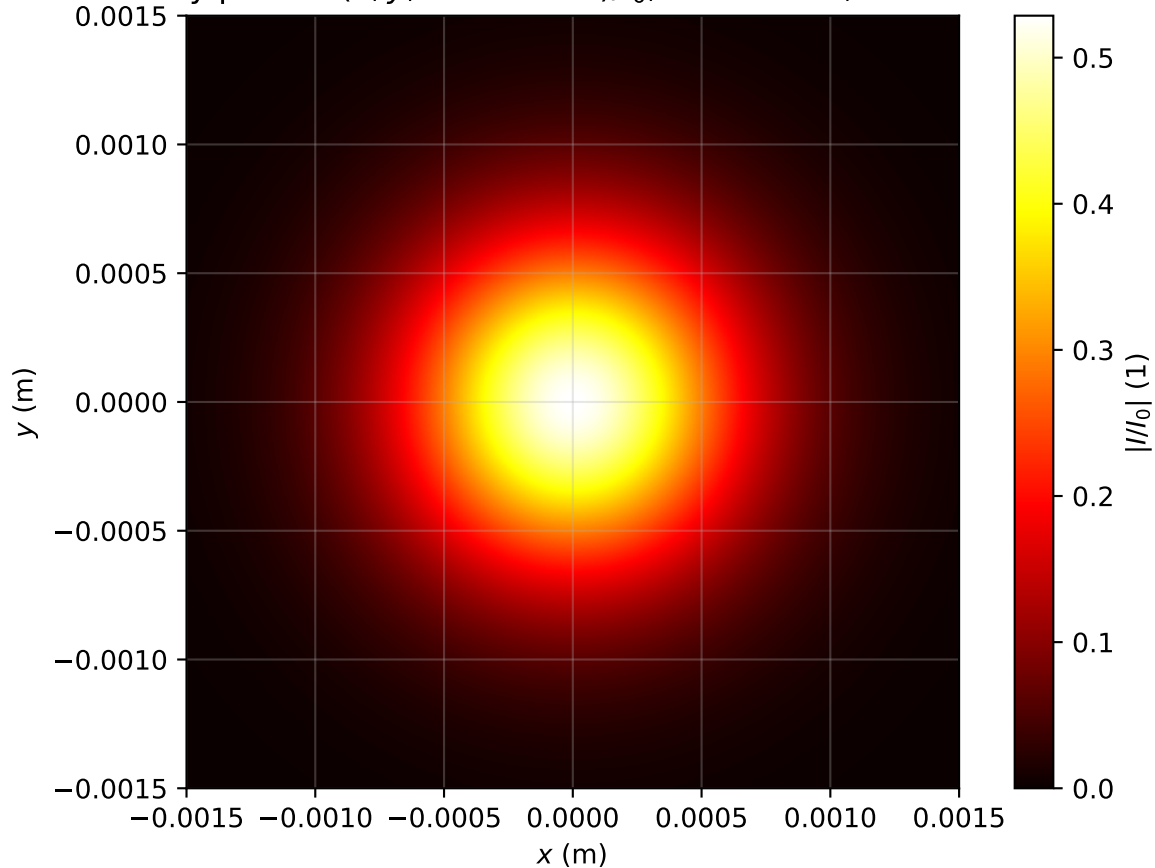
Intensity profile I(x, y, z = 2.786m)/I_0 , Pin=0.4Pcr, artificial time
